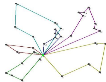
Figure 1: The optimal solution of a CVRP 39-6 problem.
