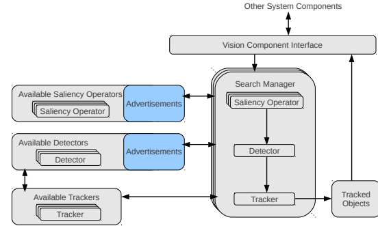
Figure 1: The processing architecture of the vision system.
