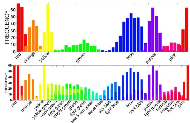
Figure 1. Frequency distributions over color labels in Experiment 1. The top panel illustrates the frequency distributions over the 7 most frequent colors labels. Each bar represents a 5 unit range on the hue scale from 0-239. The colors are presented below the corresponding hue values. The bottom panel illustrates the frequency distributions over the 21 most frequent labels.
