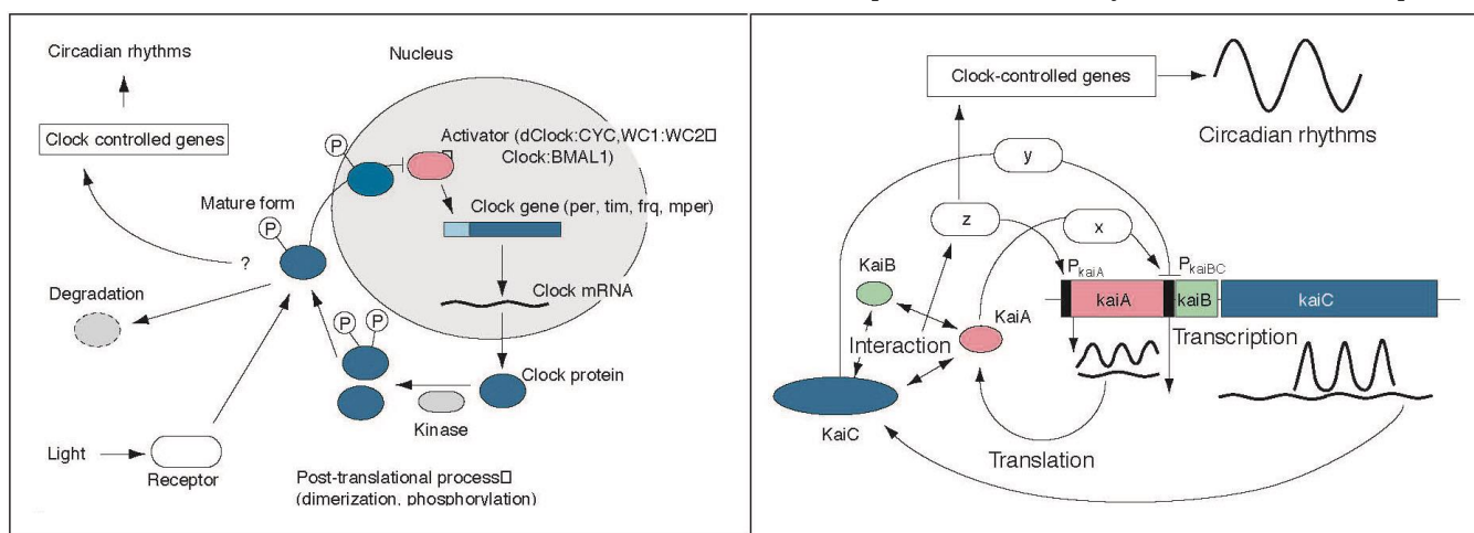
Figure 1: Kondo & Ishiura’s (1999) Figures 3 (left) & 4 (right). At left is the TTFL model of rhythmicity in eukaryotic cells. At right, available data in S. elongatus are fitted into a similar scheme. See text for discussion.
