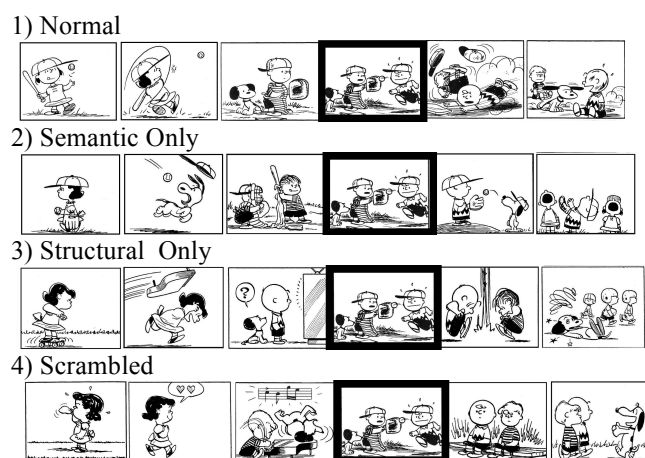
Figure 2: Example Stimuli.
