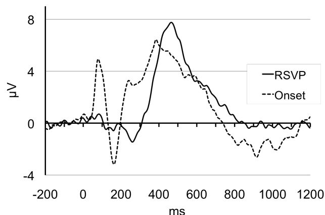
Figure 1: Human ERP for targets in RSVP and Onset presentation averaged across P7 and P8 electrode locations. ERPs are time-locked to target presentation time 'T'.
