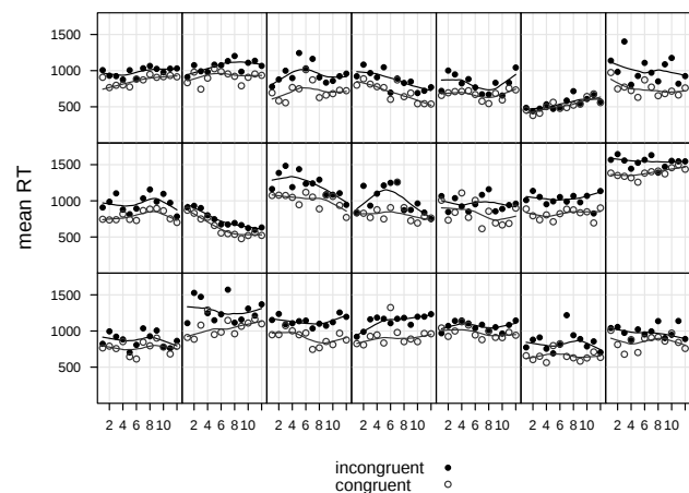
Figure 3: Mean raw response times per subject for congruent vs. incongruent trials across 12 blocks of 40 trials. In each panel, non-parametric regression lines are plotted for congruent vs. incongruent trials.
