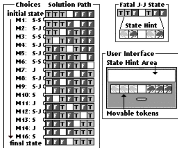
Figure 1: The Toads and Frogs problem
