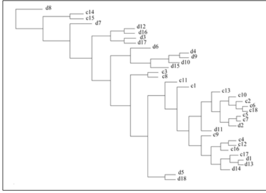
Figure 2. Cluster analysis performed on the activation patterns of the network's hidden units for cats (c1-c18) and dogs (d1-d18). Distances and cluster structure in this graph correspond to the overall similarity structure of the network's internal representations of the input patterns.
